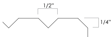
VU VERSO PROFILE DETAIL
