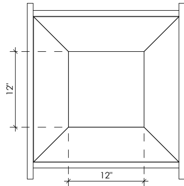
QUI DIMENSIONS (NOMINAL) WEIGHT: 3 LBS
