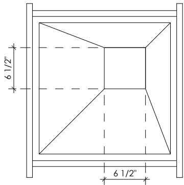
VEDI DIMENSIONS (NOMINAL) WEIGHT: 3 LBS
