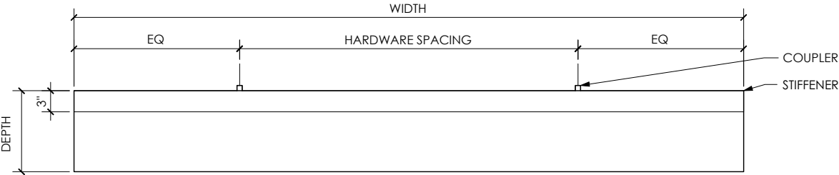
QUADRO ELEVATION - FRONT 95" x 11.5" SHOWN
