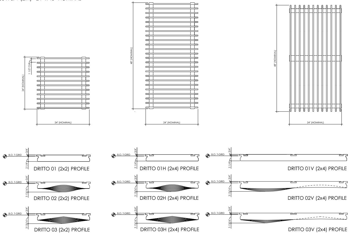
DRITTO 01- 03 DIMENSIONS
