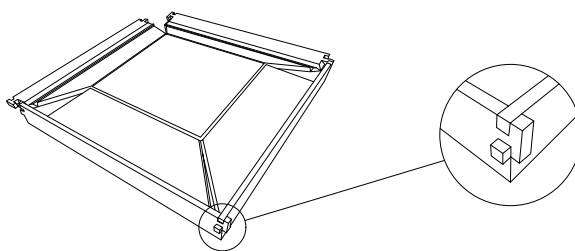
INTERLOCK CORNERS
