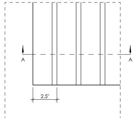
DETAIL: 2.4" PLANKS
